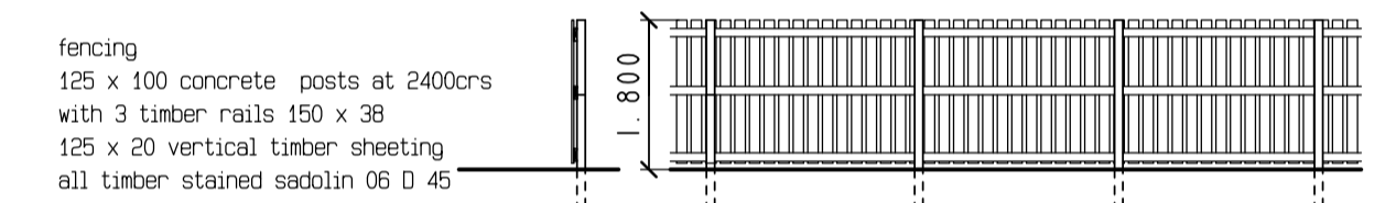
fencing type A scale 1 : 100
