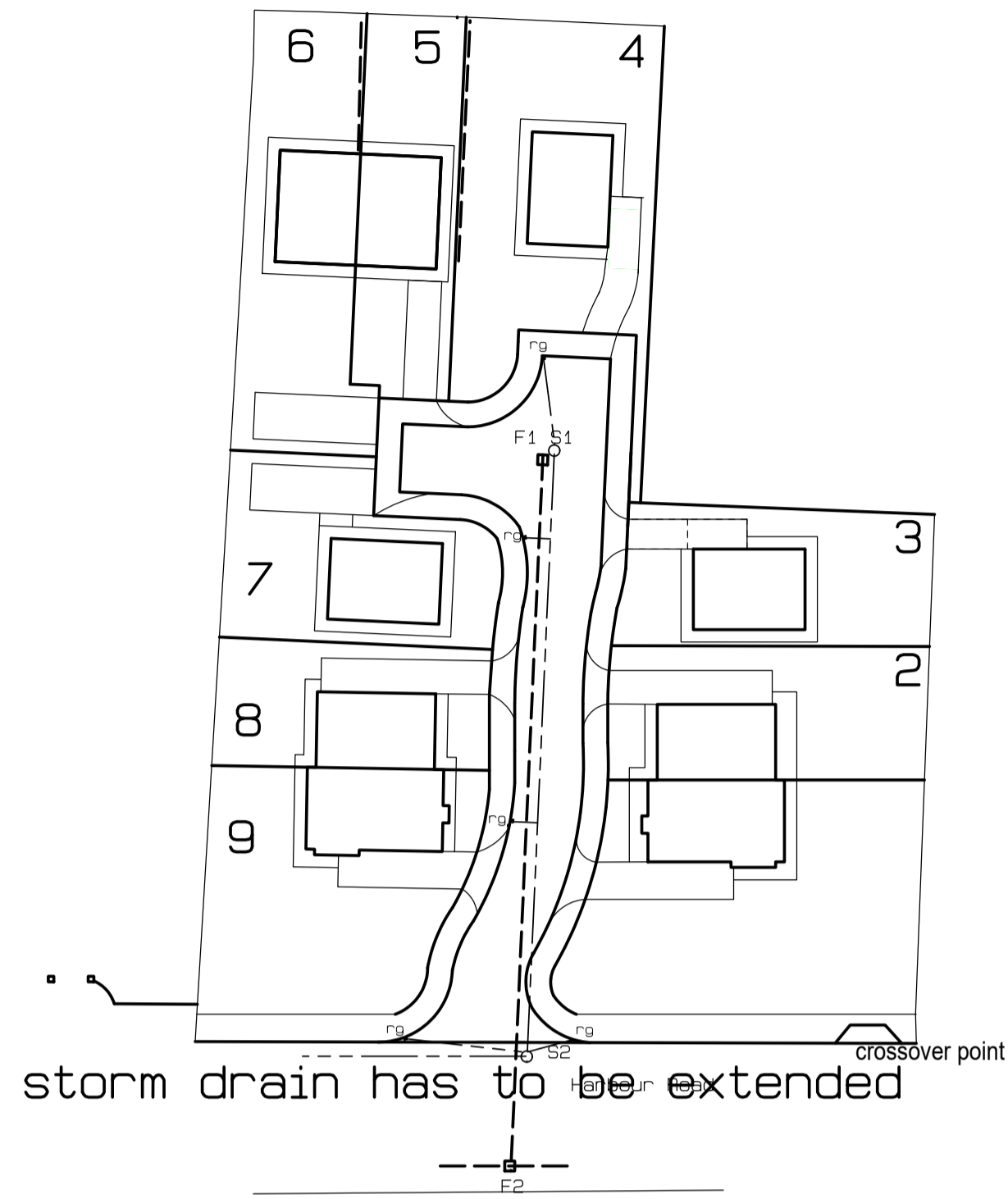
storm and foul drainage layout scale 1 : 500
