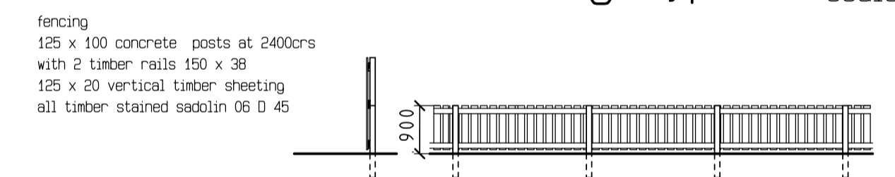
fencing type B scale 1 : 100
