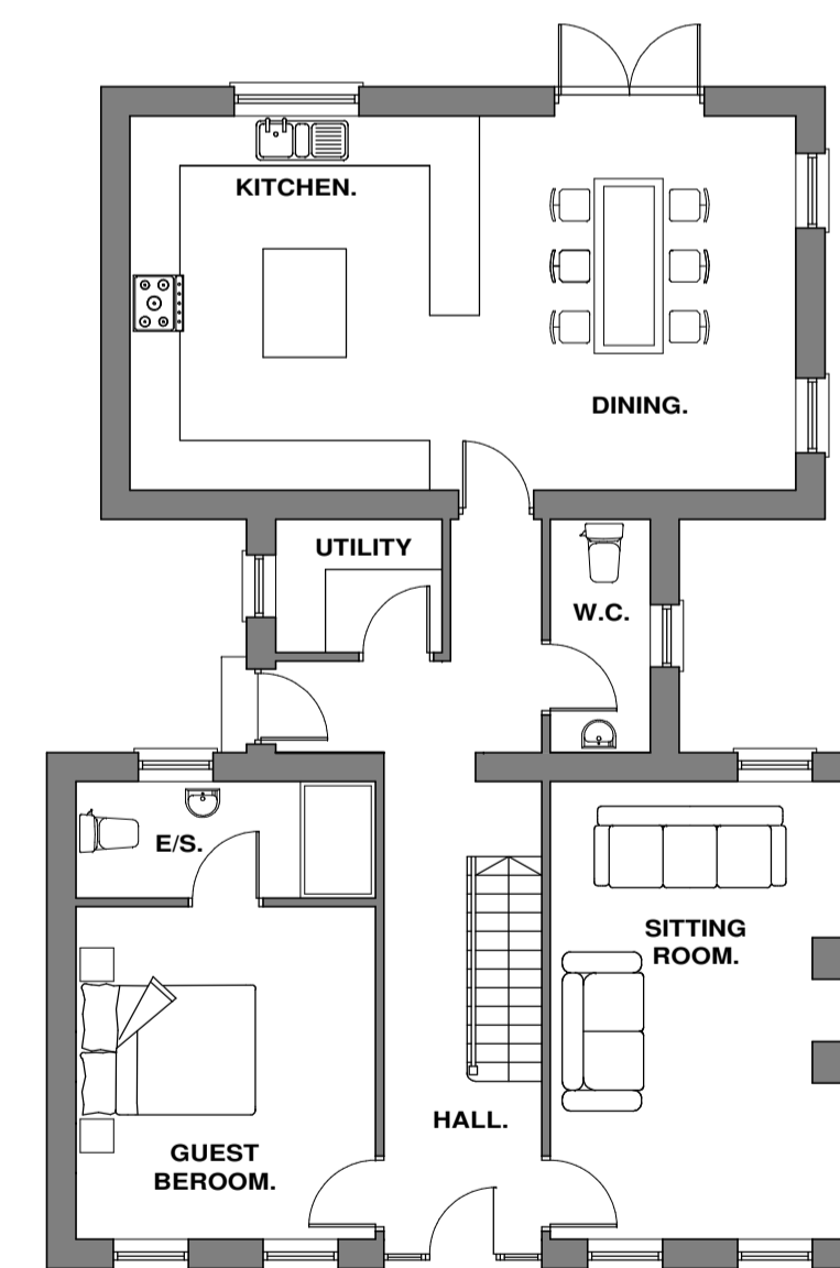
PROPOSED GROUND FLOOR LAYOUT 1-100.
